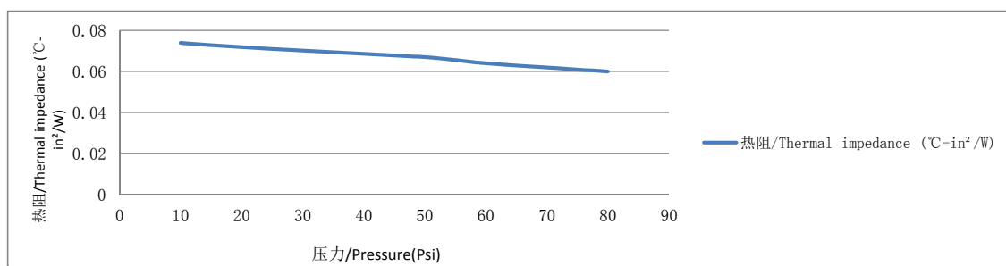
产品的FDTr曲线图 Graph of thermal resistance of product
