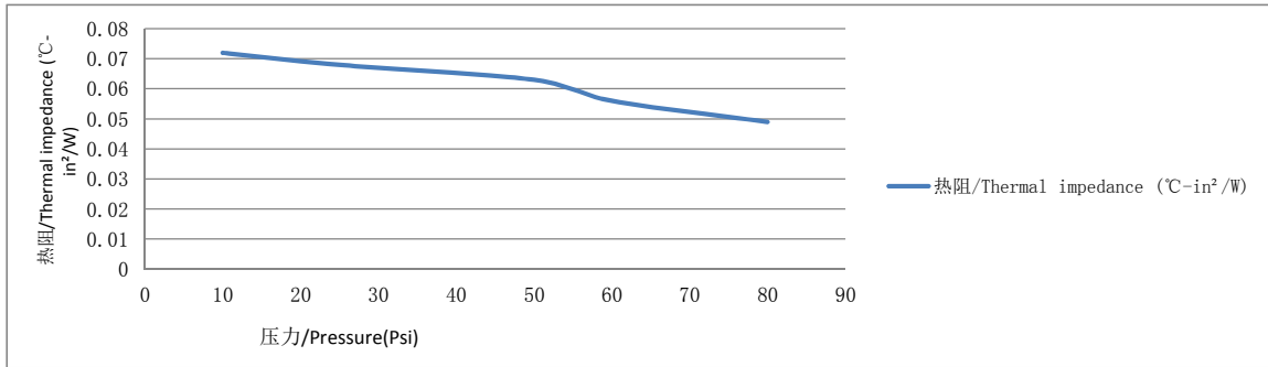
产品的FDTr曲线图 Graph of thermal resistance of product
